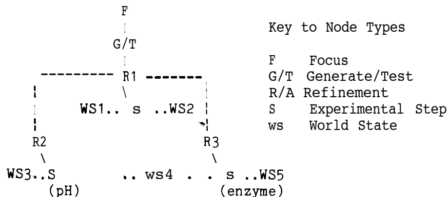
Figure 8. Planning Network for Enzyme/pH Example
