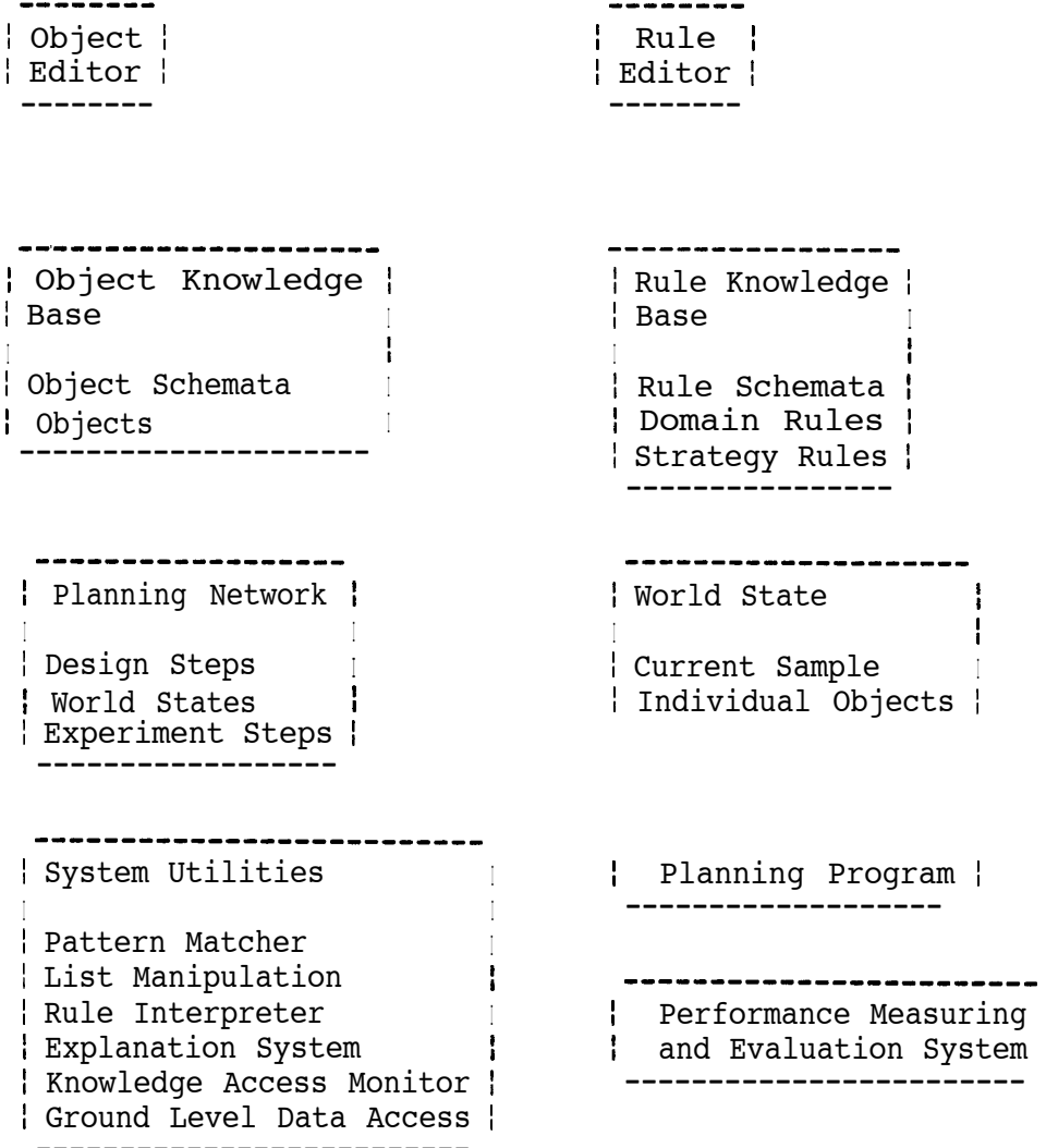
Figure 4. MOLGEN System Components
