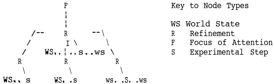
Figure 7. Fragment of Planning Network During Hierarchical Planning
